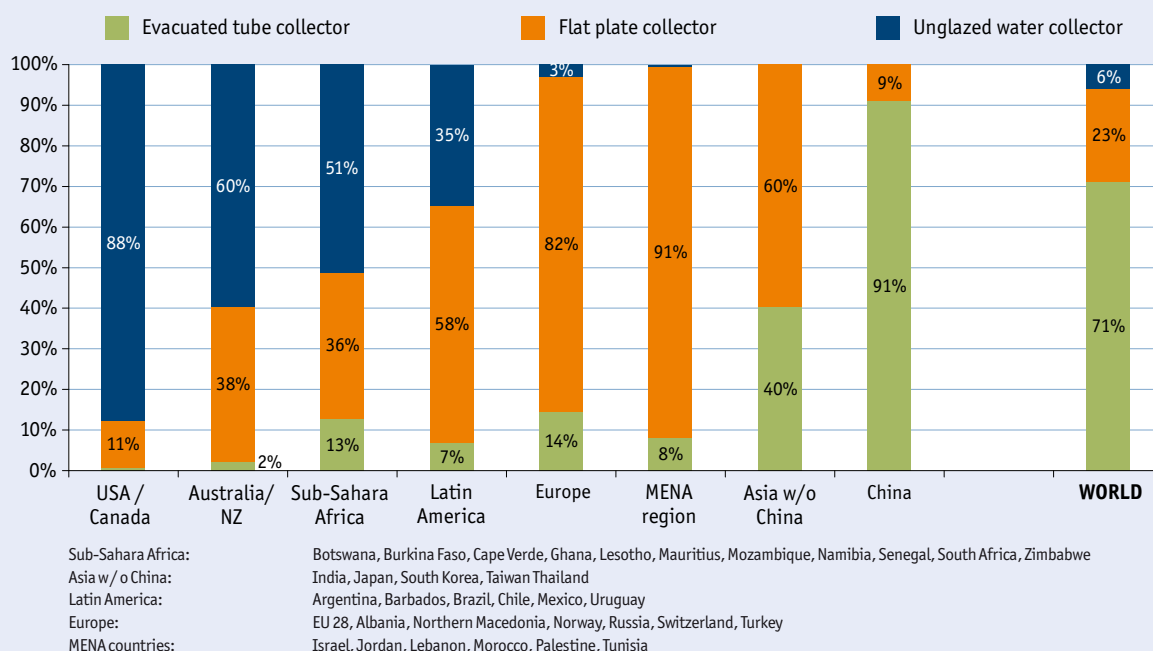
Figure 52: Distribution by type of solar thermal collector for the total installed water collector capacity in operation by the end of 2017
