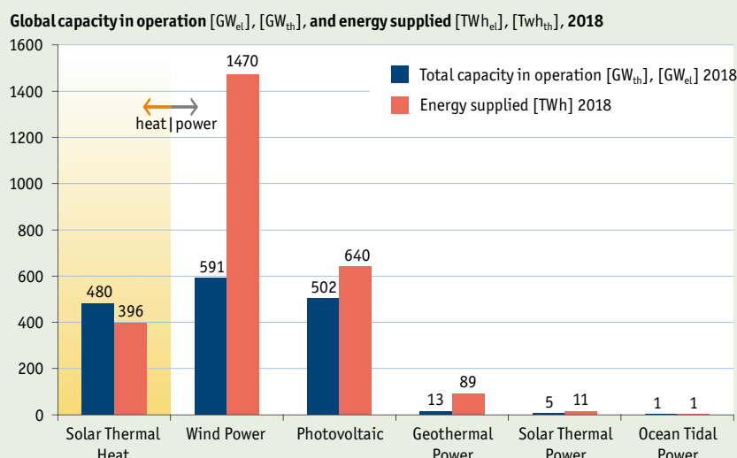
Figure 3: Global capacity in operation [ GW_{el} ], [ GW_{th} ] 2018 and annual energy yields [ TWh_{el} ], [ TWh_{th} ]. (Sources: AEE INTEC, Global Wind Energy Council (GWEC), European PV Industry Association (EPIA), REN21 - Global Status Report 2019)
