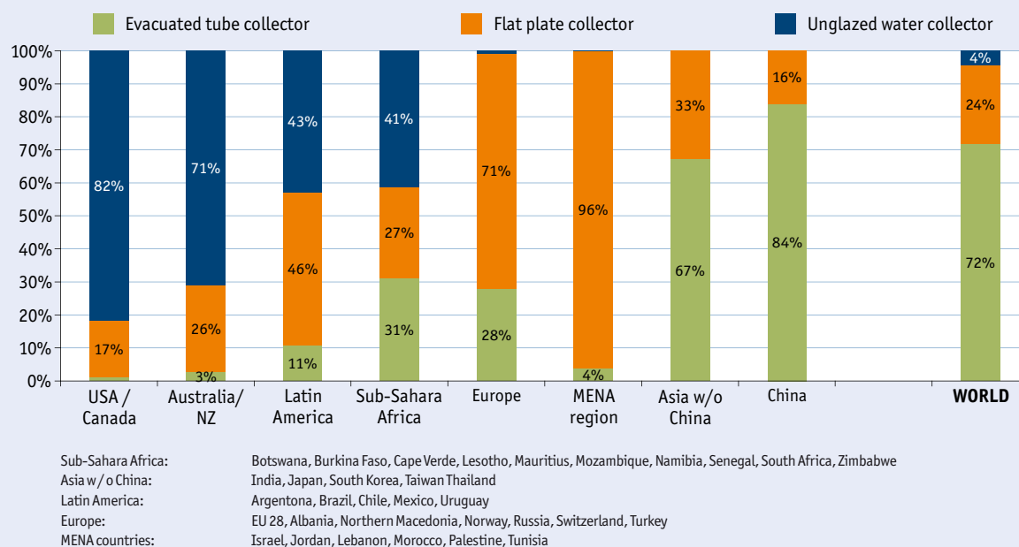
Figure 53: Distribution by type of solar thermal collector for the newly installed water collector capacity in 2017
