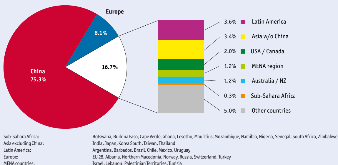
Figure 33: Share of newly installed capacity (glazed and unglazed water and air collectors) by economic regions in 2017
