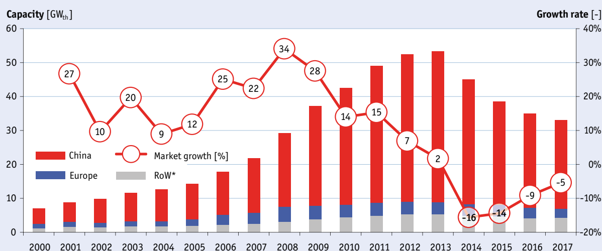
Figure 42: Global market development of glazed water collectors from 2000 to 2017
