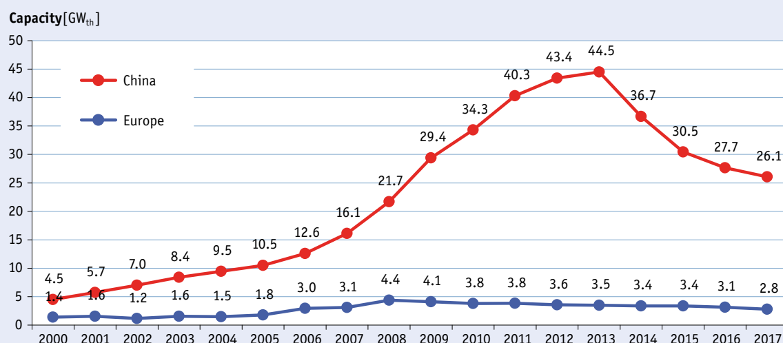
Figure 43: Market development of glazed water collectors in China and Europe 2000 – 2017
