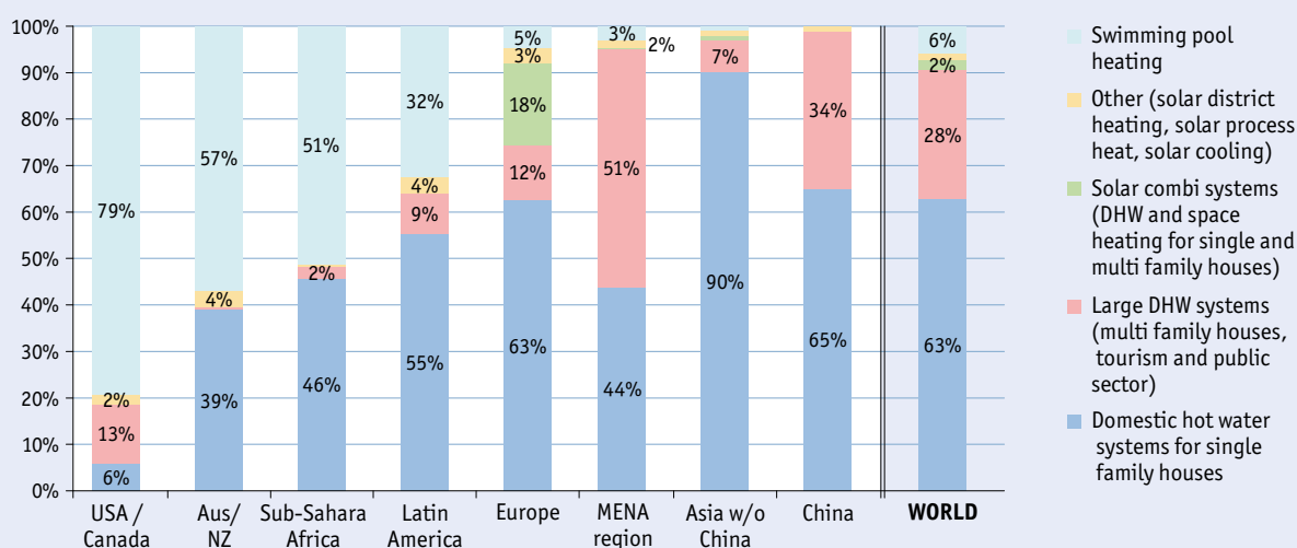
Figure 56: Distribution of solar thermal systems by application for the total installed water collector capacity by economic region in operation by the end of 2017
