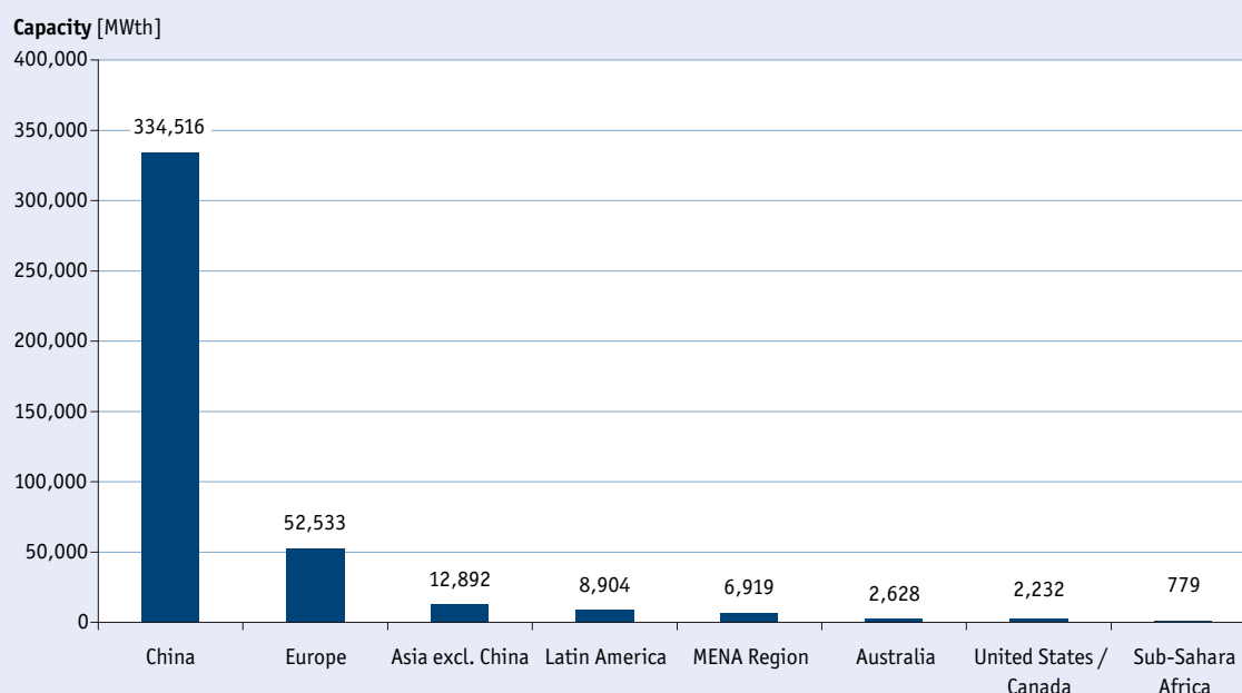
Figure 29: Total capacity of glazed flat plate and evacuated tube collectors in operation by economic region in 2017
