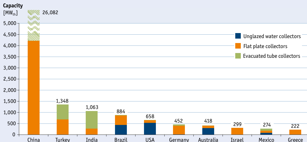
Figure 36: Top 10 markets for glazed and unglazed water collectors in 2017 (absolute figures in MW th )
