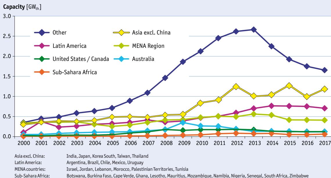
Figure 45: Market development of glazed water collectors in the Latin America, United States / Canada, Sub-Sahara Africa, Asia, the MENA Region and Australia (excluding China and Europe) from 2000 to 2017
