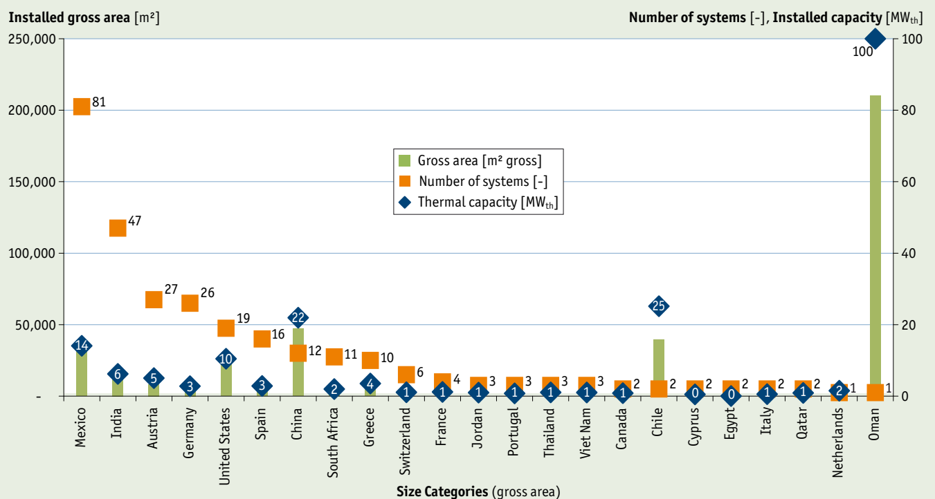
Figure 11: Global solar process heat systems in operation by end of March 2019 – countries. Only countries with at least 0.7 \text{ MW}_{\text{th}} ( 1,000 \text{ m}^2 gross area) are shown (285 of 308 systems accounting for 98% of installed thermal capacity) (Source: IEA SHC Task49/IV SHIP database)
