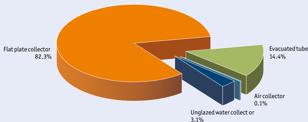
Figure 22: Distribution of the total installed capacity in operation by collector type in 2017 – EUROPE
