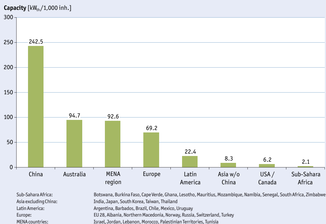
Figure 30: Total capacity of glazed flat plate and evacuated tube collectors in operation by economic region and in kW th per 1,000 inhabitants in 2017
